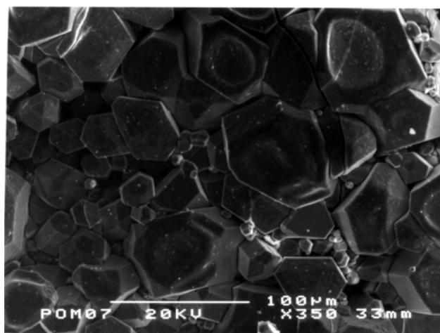
Fig. 1 SEM image of crystals of the trigonal \text{Ba}_3\text{MoN}_4 .
